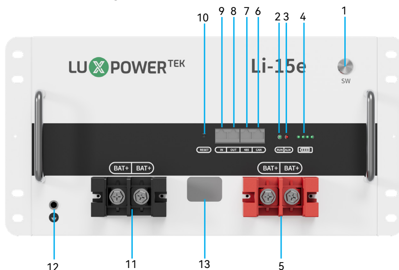
Figure 2-1 The sketch of interface.
