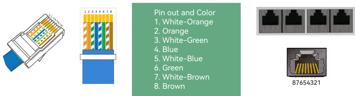
Figure 2-2 CAN, RS485, OUT, IN interface definition
