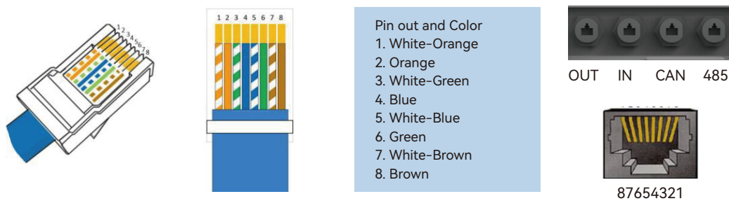
Figure 2-2 CAN, RS485, OUT, IN interface definition
