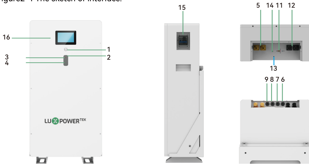
Figure2-1 The sketch of interface.
